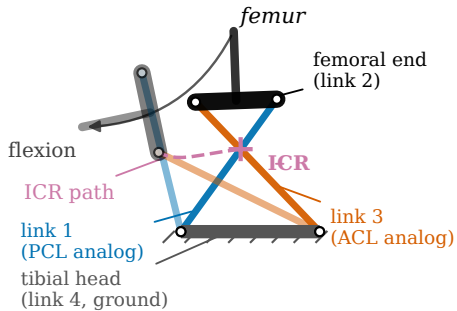
(A) Crossed four-bar knee linkage
