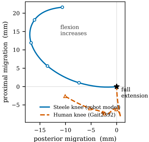
(B) ICR migration, sagittal plane
